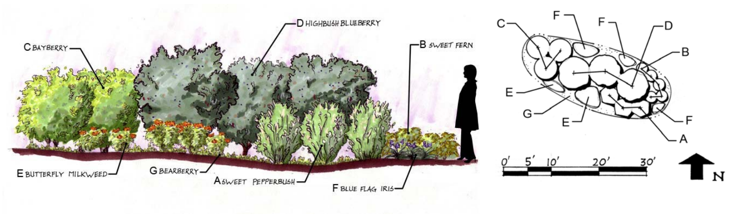
Figure 4. Rain Garden Example - Planting Plan 1
